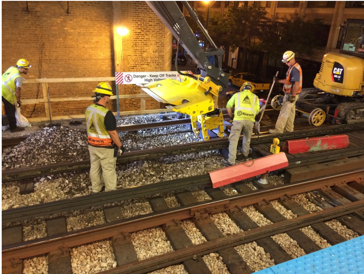
Tie installation, Track 4 Lawrence Station
