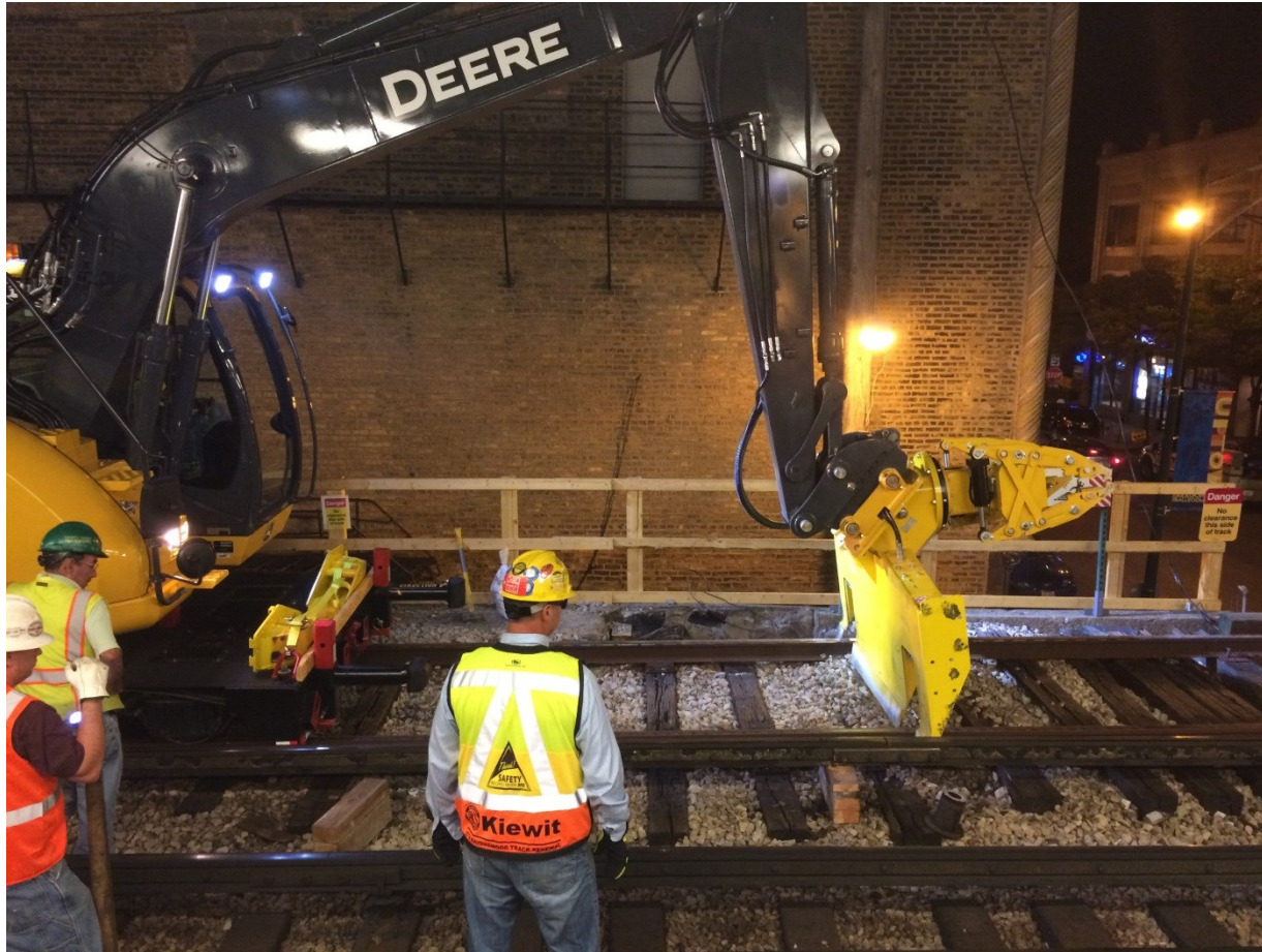
Tie demolition, Track 4 Lawrence Station
